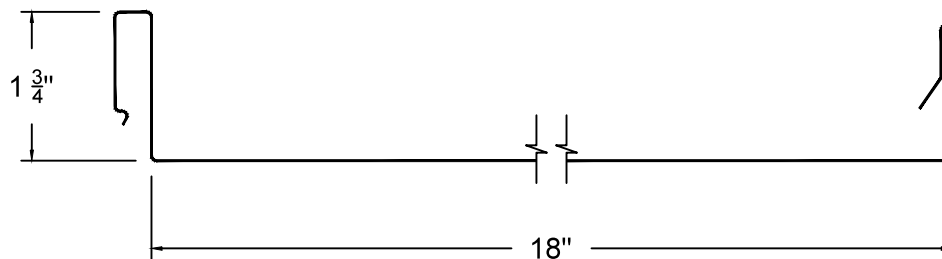
PANEL PROFILE
