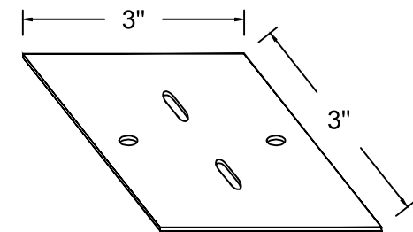
3" x 3" 18GA BEARING PLATE ISO VIEW
