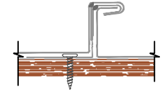
CROSS SECTION 90° SEAMING
