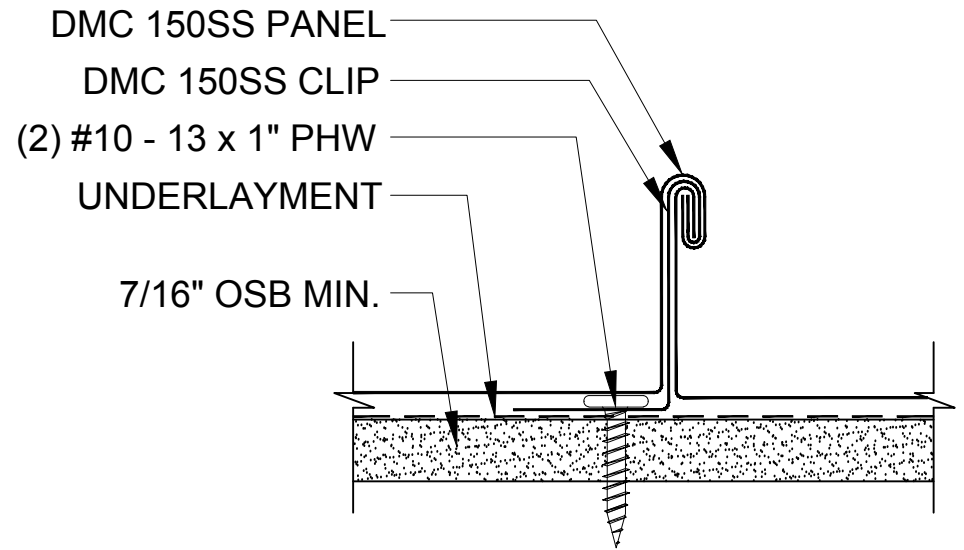
180 Degree Seam
