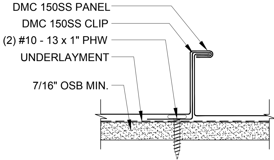
90 Degree Seam
